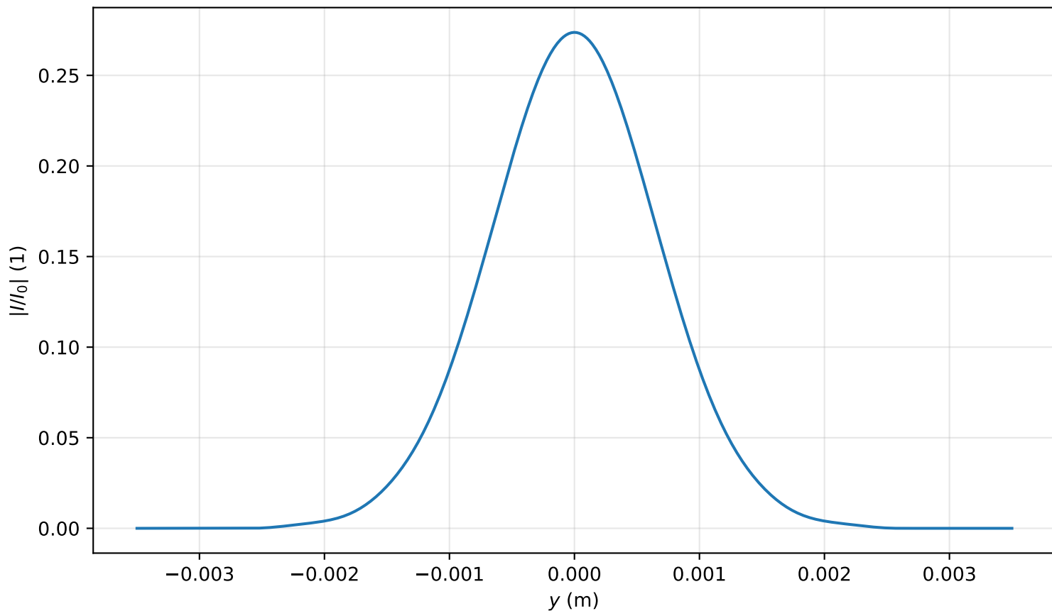
Intensity profile I(x = 0, y, z = 3.742)/I_0 , P_{in}=0.2P_{cr} , artificial time
